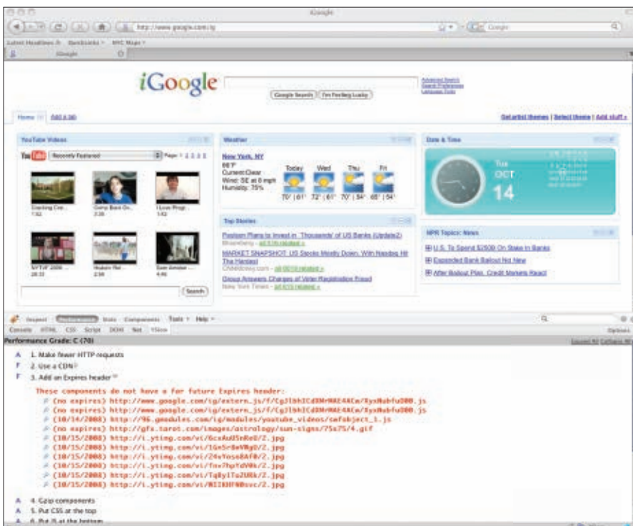
Figure 3: YSlow.
